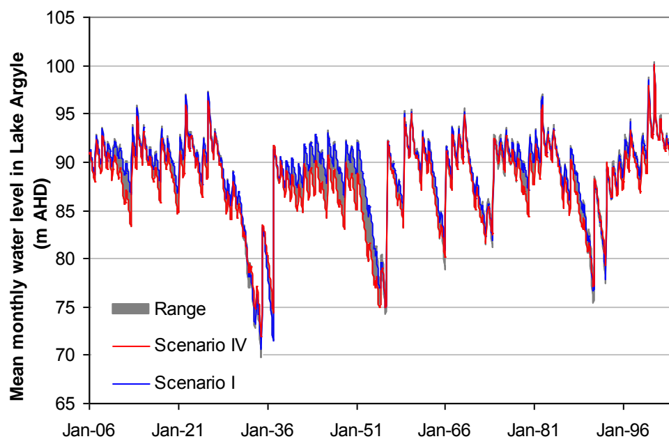
Figure 20 Variation in water level in Lake Argyle for five allocation scenarios (mean monthly)
