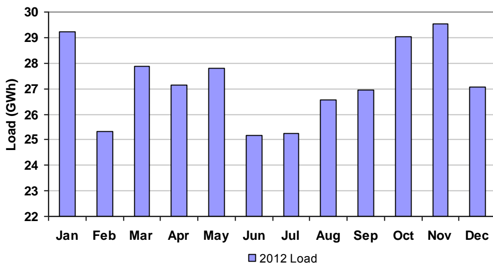
Figure 15 2012 load data input for the MIKE BASIN reservoir model
