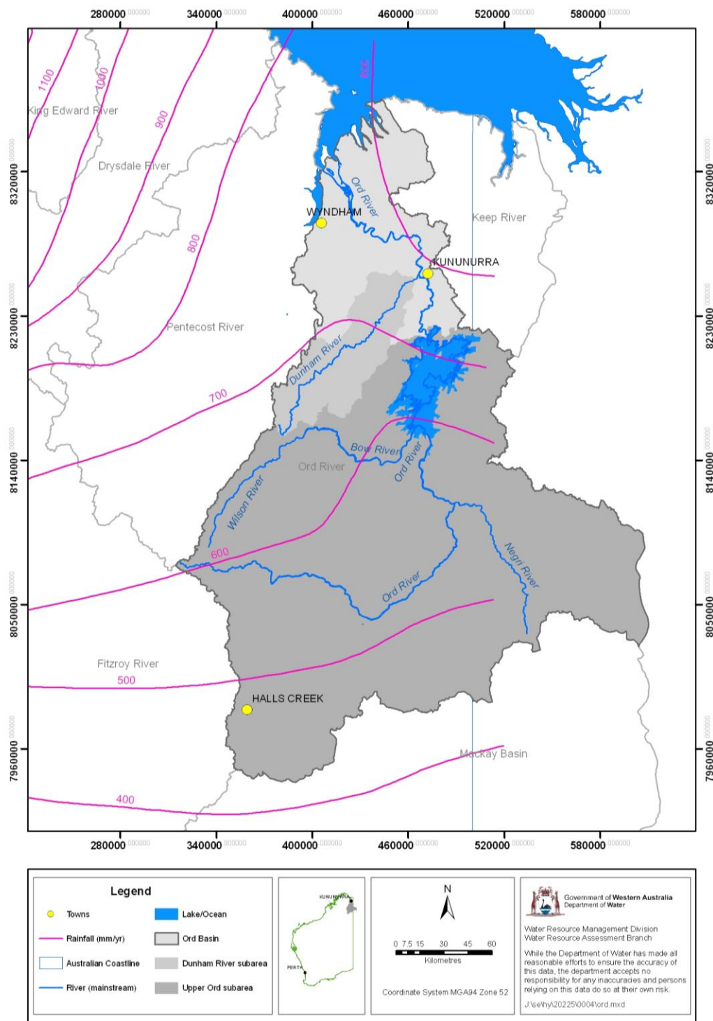
Figure 1 Ord River catchment with rainfall isohyets
