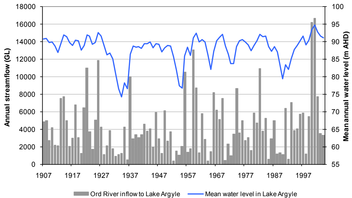
Figure 19 Comparison of inflow to Lake Argyle and water levels under the current irrigation scenario (Scenario II)
