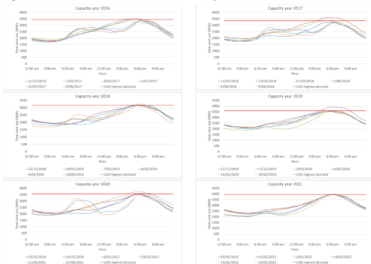
Figure 6: Load Profile on Peak Demand Days
