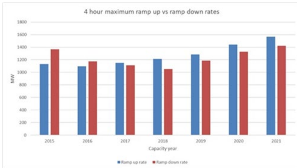
Figure 11: Maximum Ramp Up vs Ramp Down Comparison
