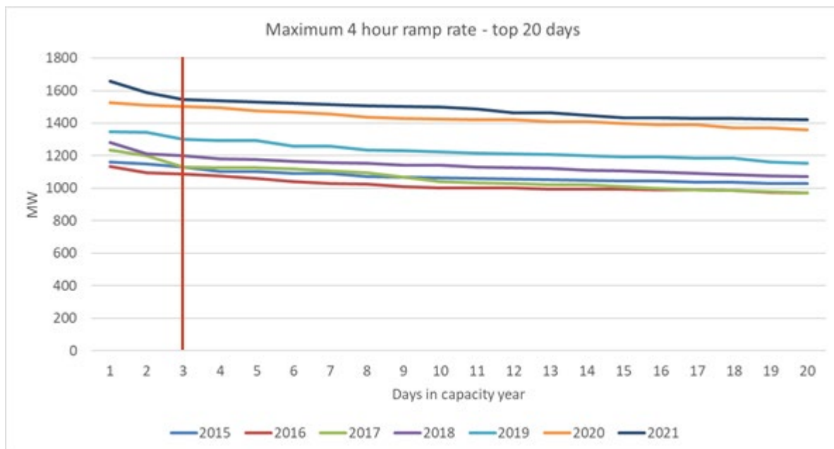
Figure 9: Maximum 4-Hour Ramp Rate Distribution – Top 20 Days
