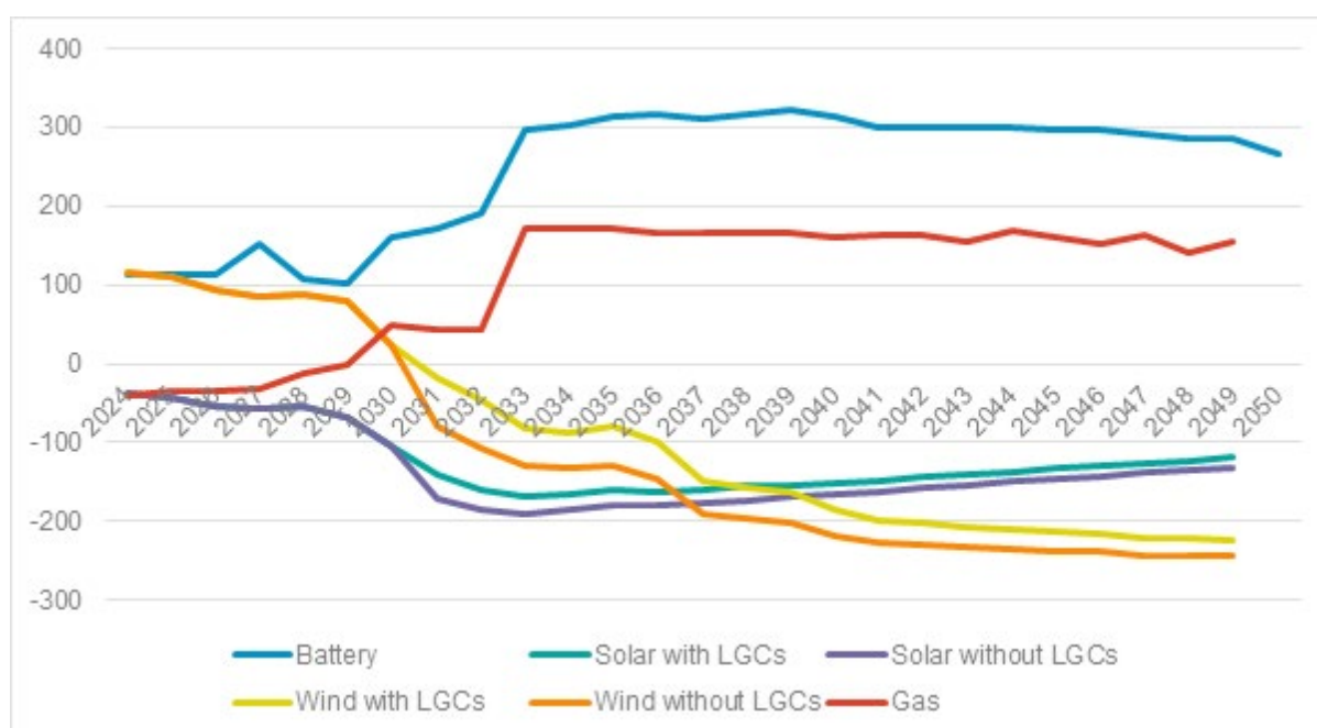
Figure 22: Profitability of New Entrant Capacity ($/kW)
