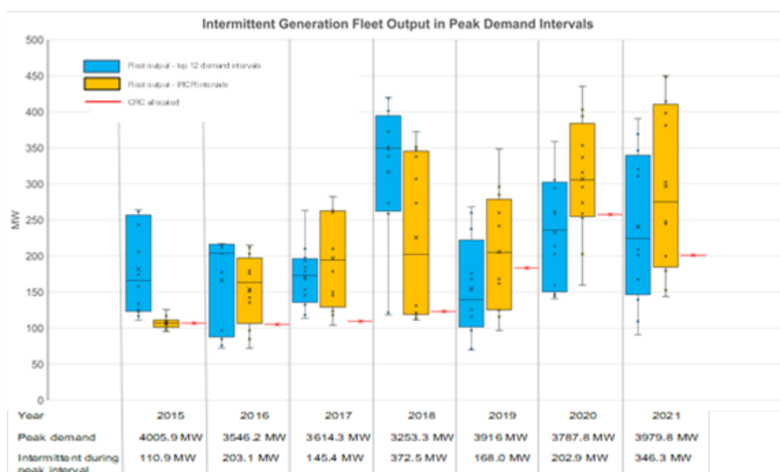
Figure 23: Intermittent Generation Fleet Output in Peak Demand Intervals
