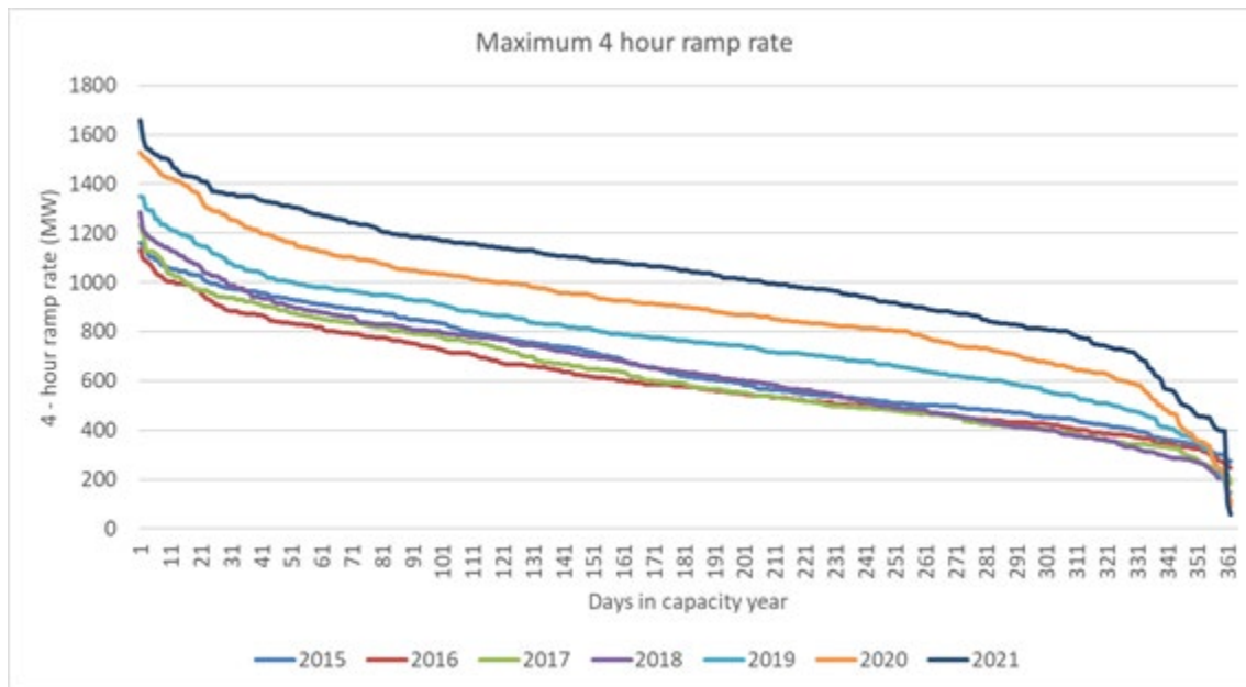
Figure 8: Maximum 4-Hour Ramp Rate Distribution
