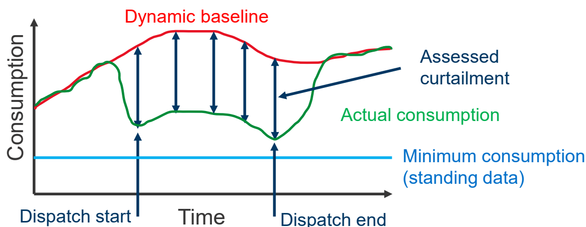
Figure 13: DSP Dispatch with a Dynamic Baseline
