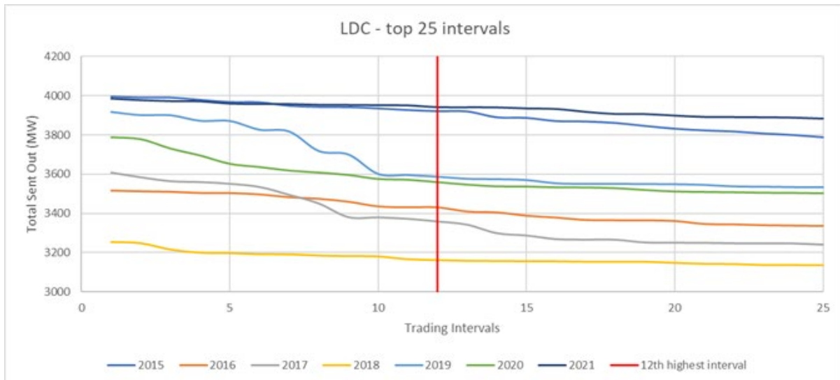
Figure 3: Load Duration Curves for 2015-2021 – top 25 Intervals
