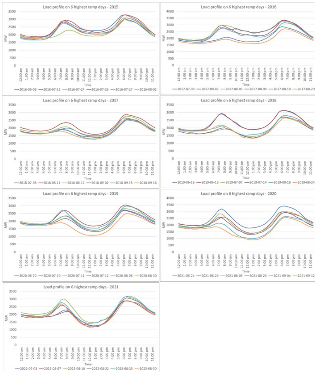
Figure 10: Load Profile on Top 6 Highest Ramp Days
